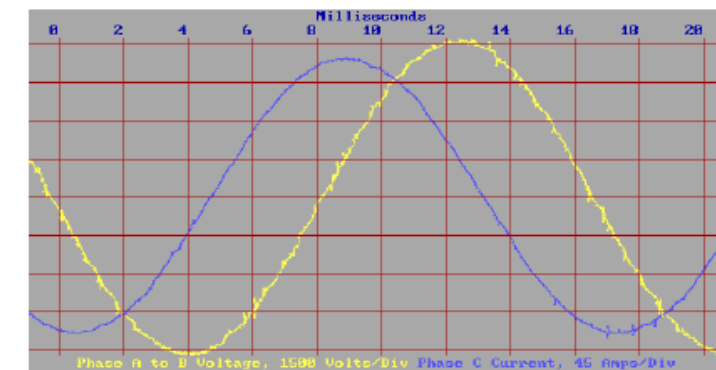
Input voltage and current waveforms
