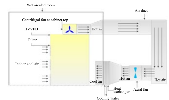
Air conditioner cooling schematic diagram
