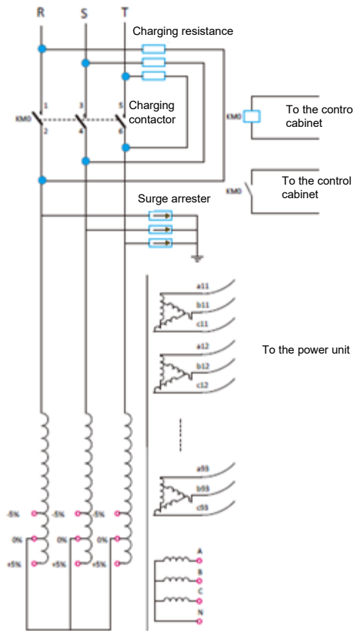
Anti-surge circuit diagram for a system
