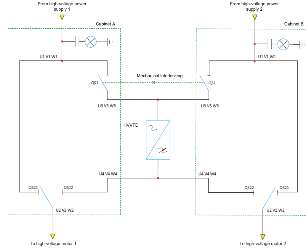
Manual one-drive-two bypass diagram
