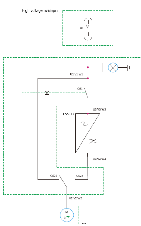
Manual one-drive-one bypass
