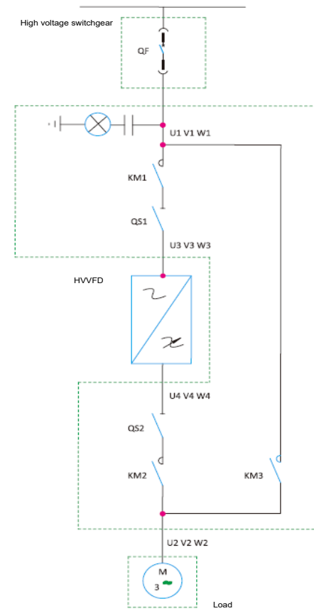
Automatic one-drive-one bypass
