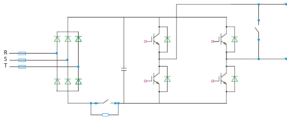
Anti-surge circuit for a unit
