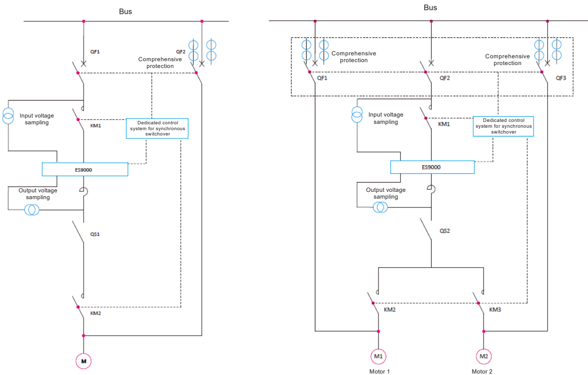
One-drive-one synchronous switchover softstart MVVFD
